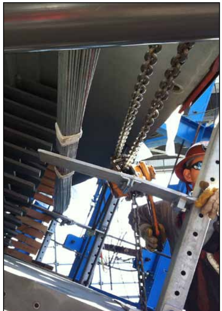
Fitting Parallel Wire Test Strand (PWS) into the Jacking Saddle
