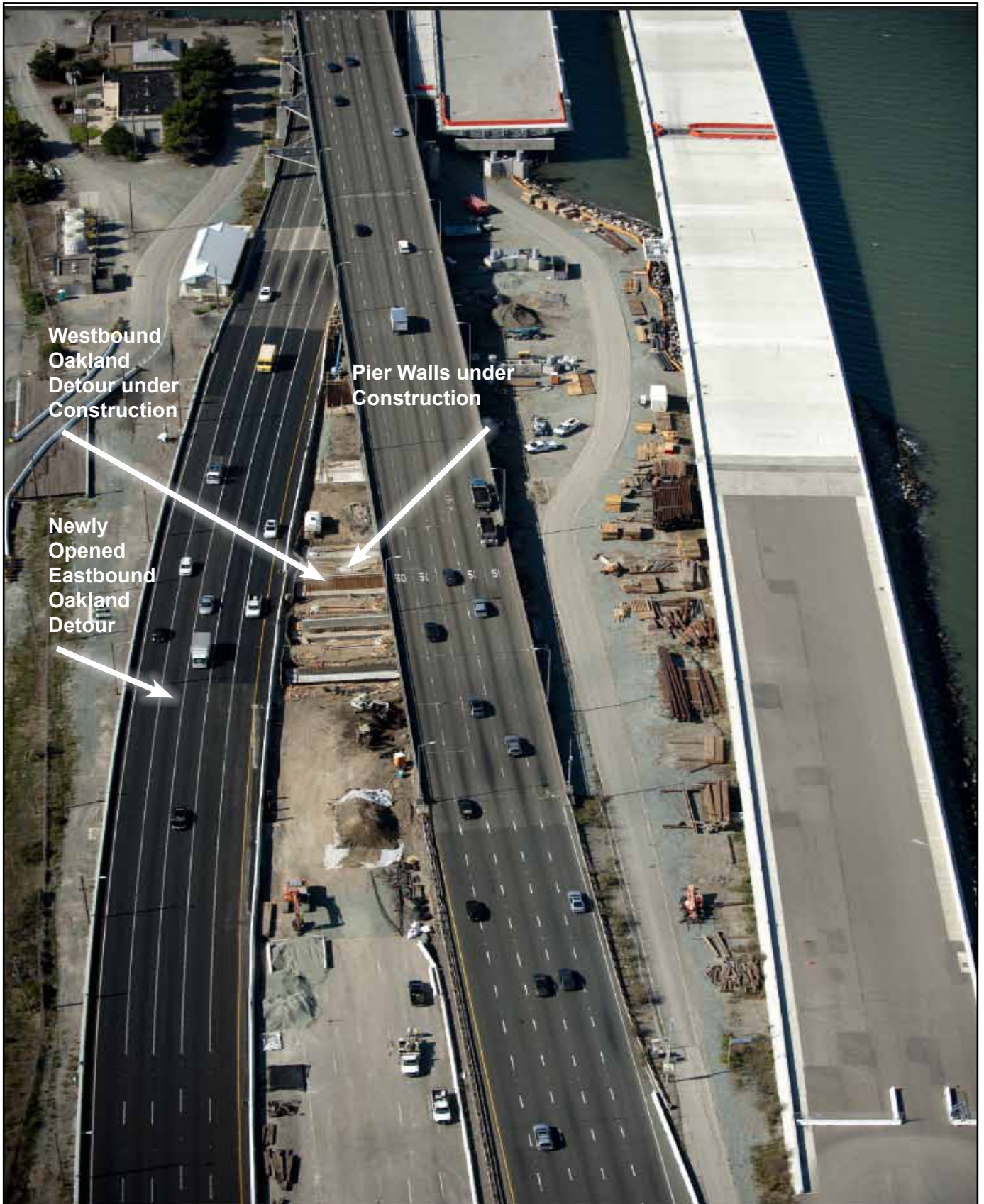
Westbound Oakland Touchdown Detour Construction Progress
