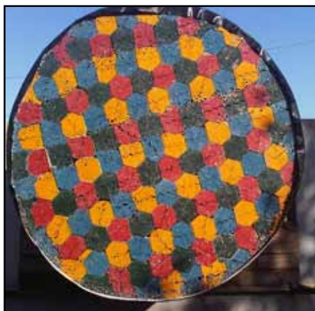
Sample of Cable Band Compaction Testing Performed at Pier 7 in Oakland
